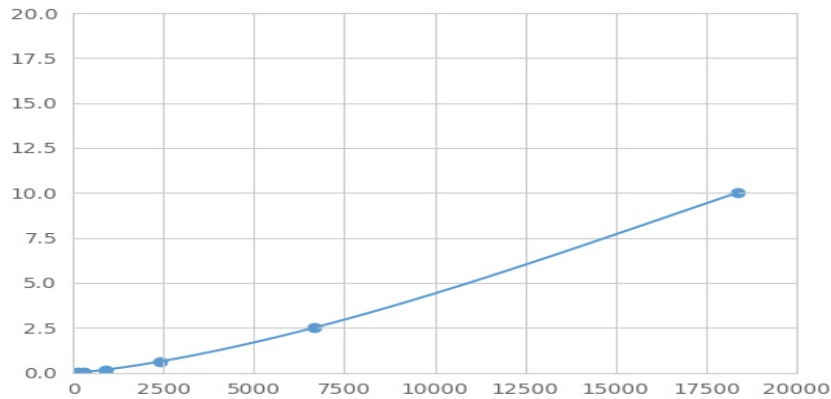
Typical Standard Curve for CAPN3 Magnetic Luminex Assay.
