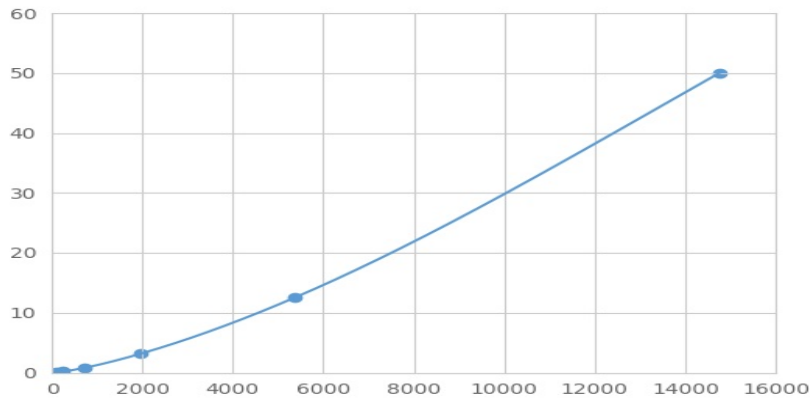
Typical Standard Curve for CRAT Magnetic Luminex Assay.
