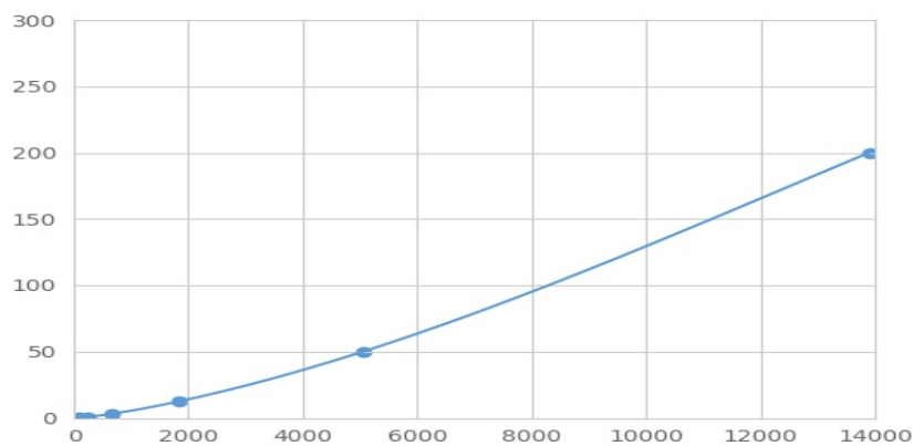
Typical Standard Curve for CSN3 Magnetic Luminex Assay.
