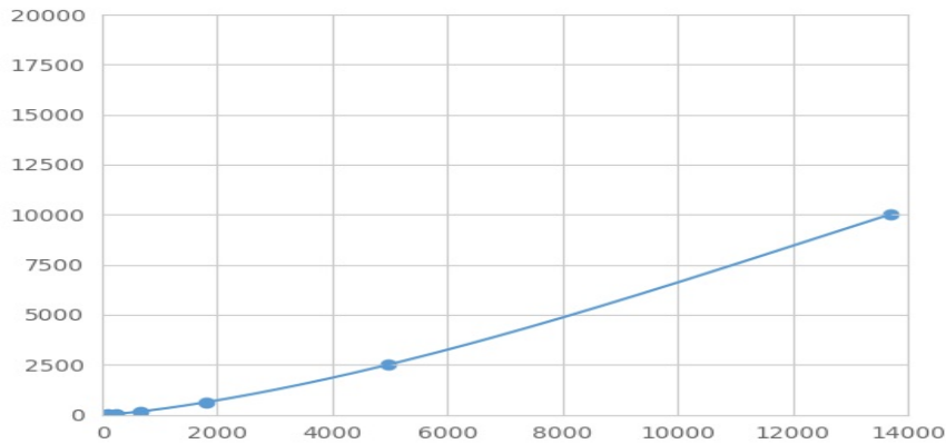
Typical Standard Curve for CASP12 Magnetic Luminex Assay.
