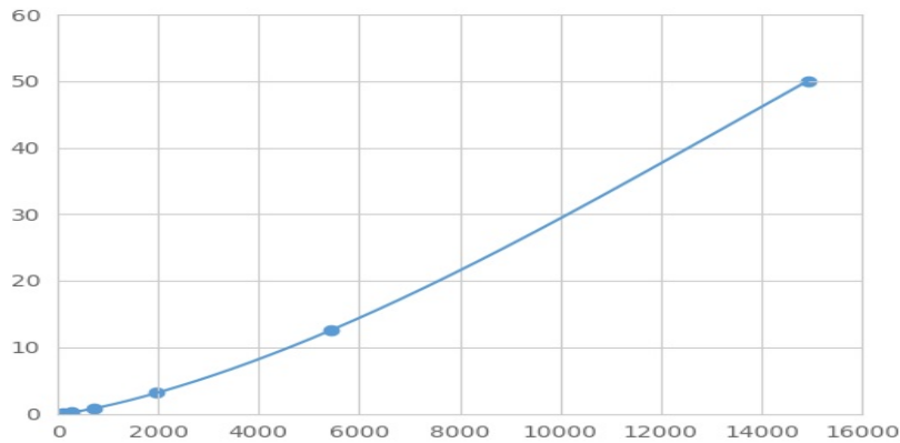
Typical Standard Curve for CHR3 Magnetic Luminex Assay.
