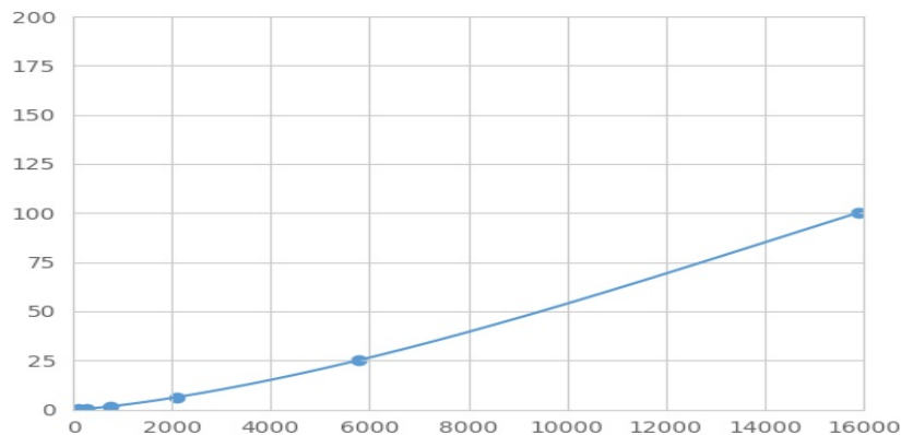
Typical Standard Curve for CS Magnetic Luminex Assay.
