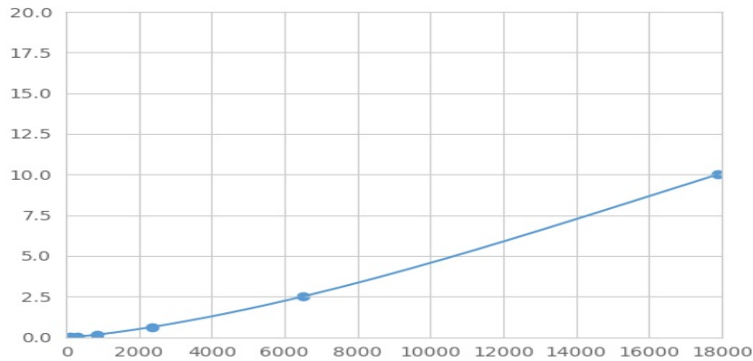
Typical Standard Curve for CD19 Magnetic Luminex Assay.
