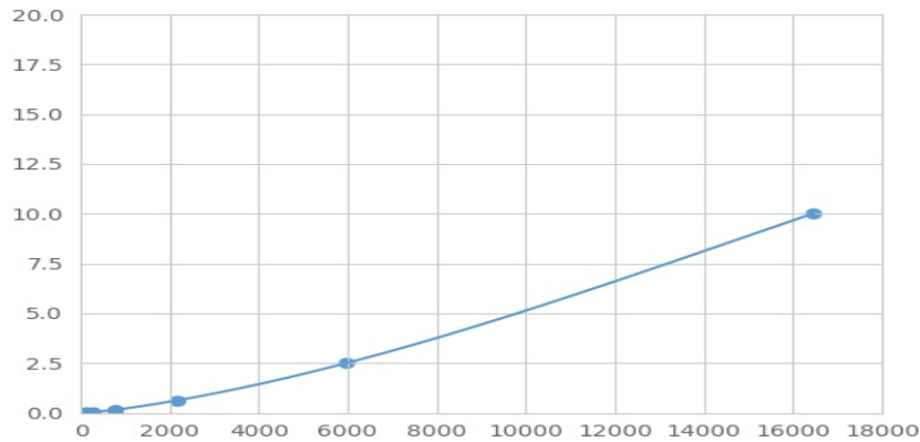
Typical Standard Curve for CD36 Magnetic Luminex Assay.
