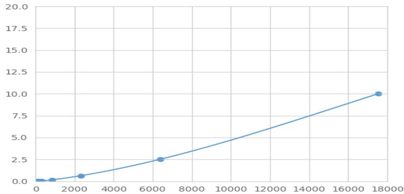
Typical Standard Curve for CART Magnetic Luminex Assay.
