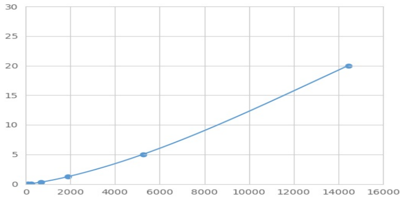
Typical Standard Curve for CSDE1 Magnetic Luminex Assay.
