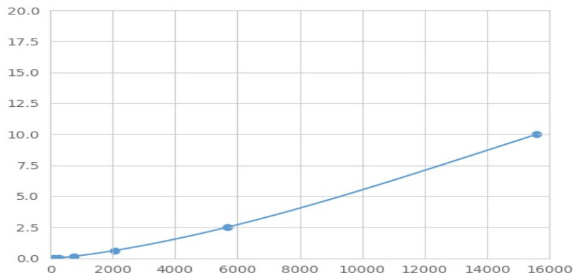
Typical Standard Curve for COL1a2 Magnetic Luminex Assay.
