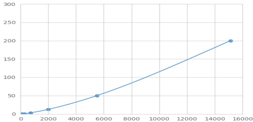
Typical Standard Curve for COL7 Magnetic Luminex Assay.
