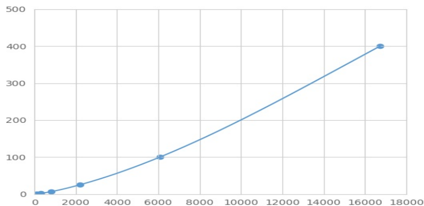
Typical Standard Curve for C4 Magnetic Luminex Assay.
