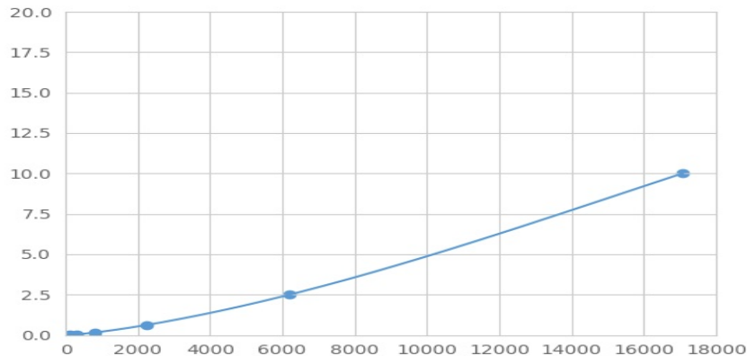
Typical Standard Curve for ConA Magnetic Luminex Assay.
