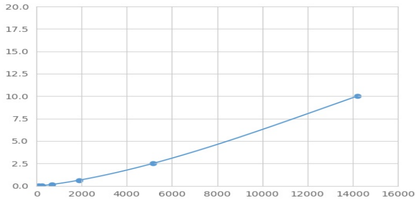
Typical Standard Curve for CX43 Magnetic Luminex Assay.
