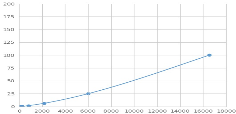
Typical Standard Curve for CYPA Magnetic Luminex Assay.
