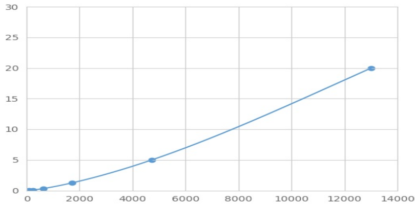
Typical Standard Curve for CSTB Magnetic Luminex Assay.
