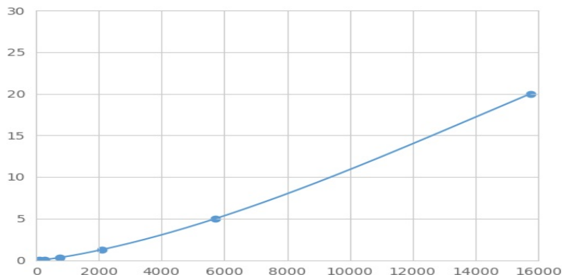
Typical Standard Curve for COX3 Magnetic Luminex Assay.
