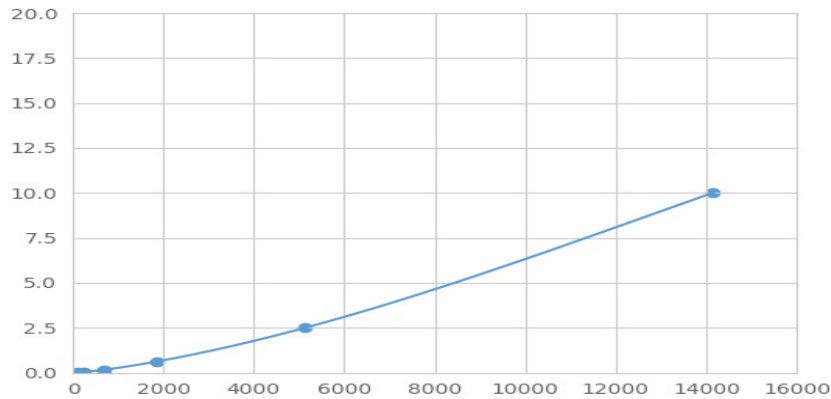
Typical Standard Curve for COX4I2 Magnetic Luminex Assay.
