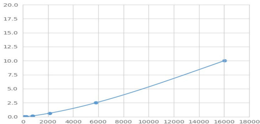
Typical Standard Curve for CYP26A1 Magnetic Luminex Assay.
