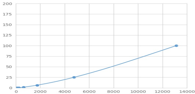
Typical Standard Curve for CYP3A5 Magnetic Luminex Assay.
