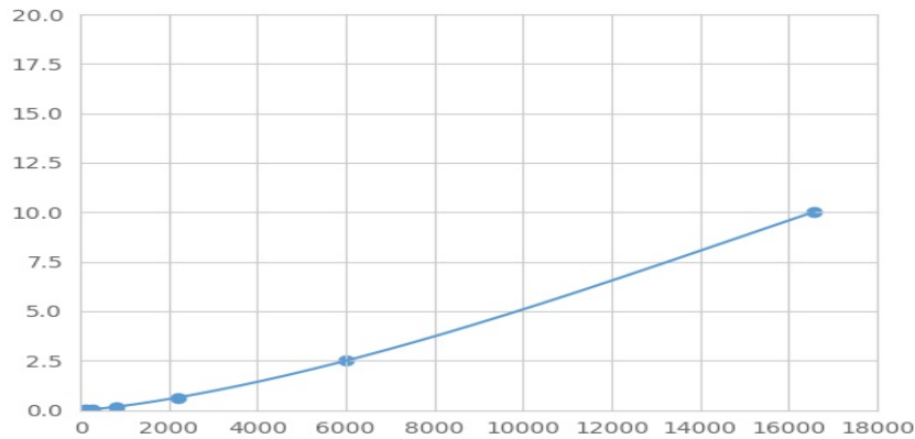
Typical Standard Curve for CK1 Magnetic Luminex Assay.
