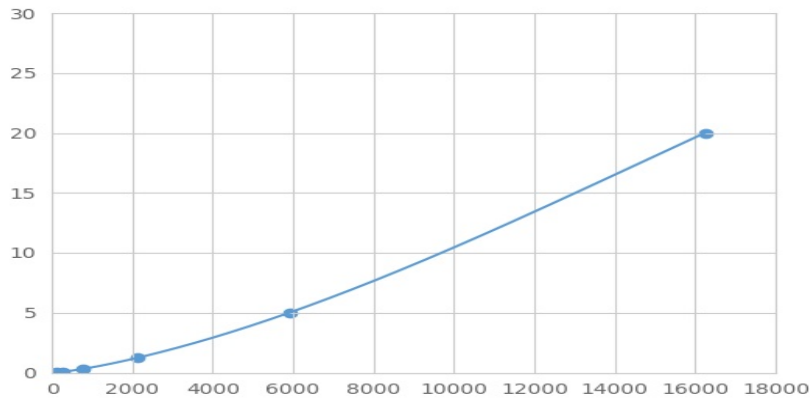
Typical Standard Curve for CK19 Magnetic Luminex Assay.
