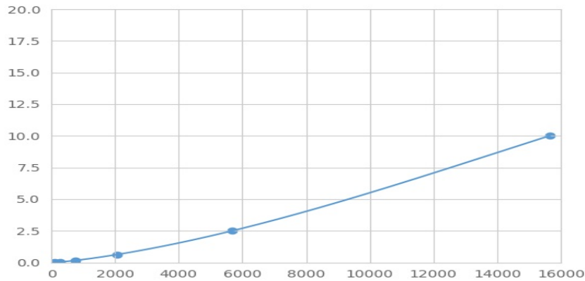
Typical Standard Curve for CK8 Magnetic Luminex Assay.
