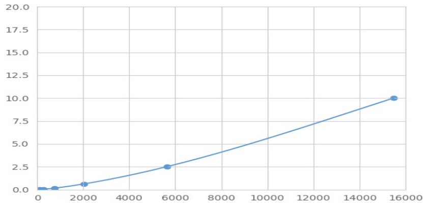
Typical Standard Curve for RAD50 Magnetic Luminex Assay.
