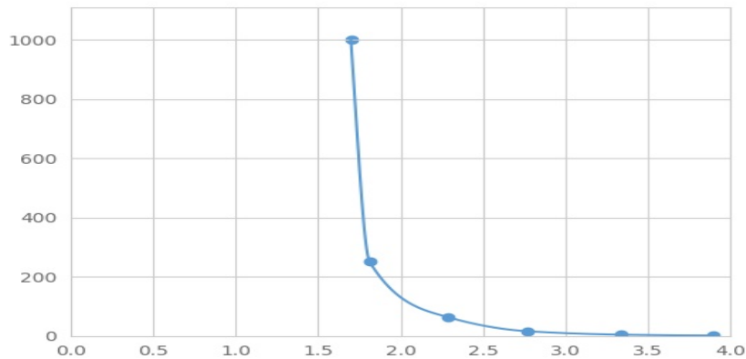
Typical Standard Curve for PP Magnetic Luminex Assay.
