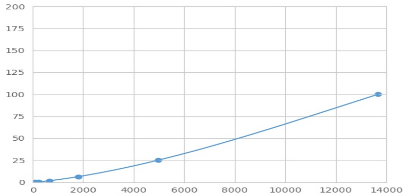
Typical Standard Curve for DDR2 Magnetic Luminex Assay.
