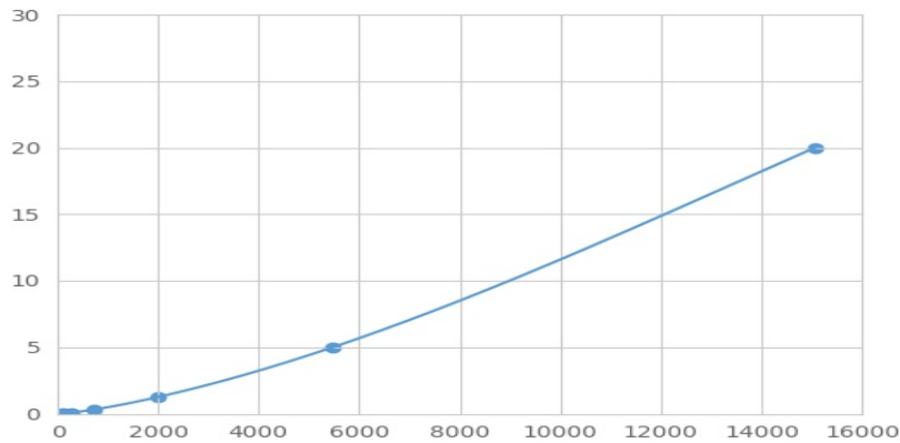
Typical Standard Curve for DLG3 Magnetic Luminex Assay.
