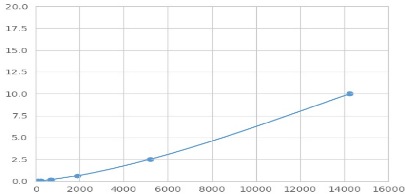
Typical Standard Curve for E2F1 Magnetic Luminex Assay.
