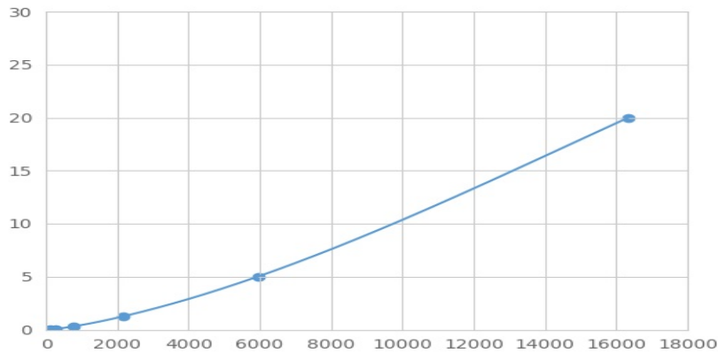
Typical Standard Curve for ELAVL1 Magnetic Luminex Assay.
