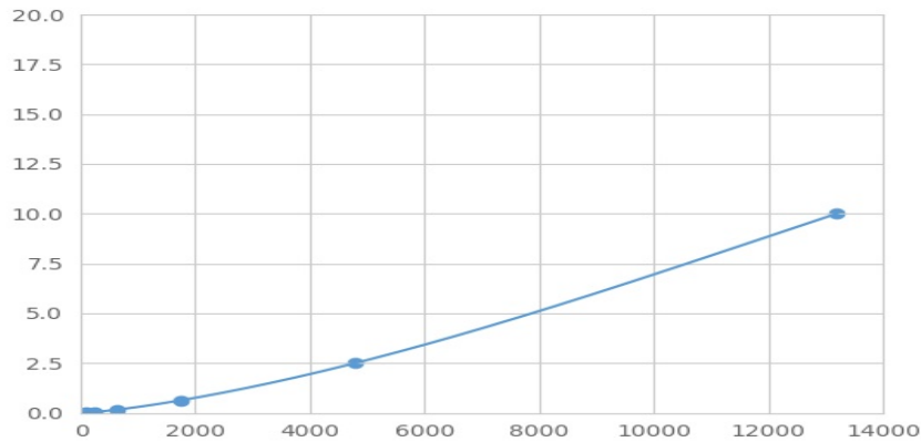
Typical Standard Curve for ETFa Magnetic Luminex Assay.
