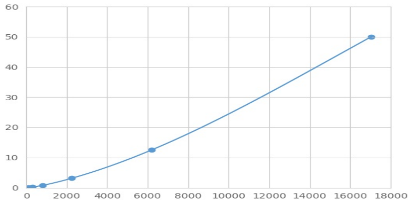
Typical Standard Curve for ENG Magnetic Luminex Assay.
