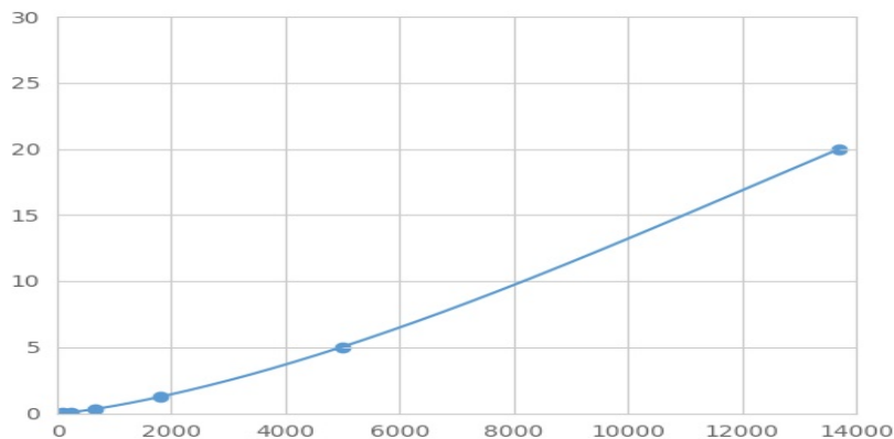
Typical Standard Curve for ERLIN1 Magnetic Luminex Assay.
