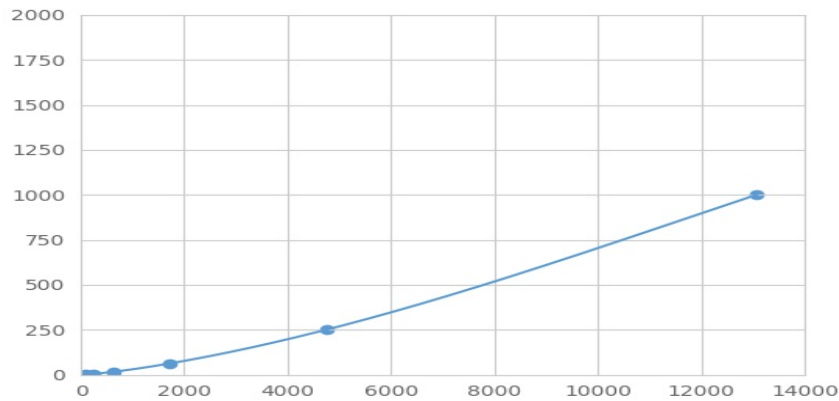
Typical Standard Curve for ECF Magnetic Luminex Assay.
