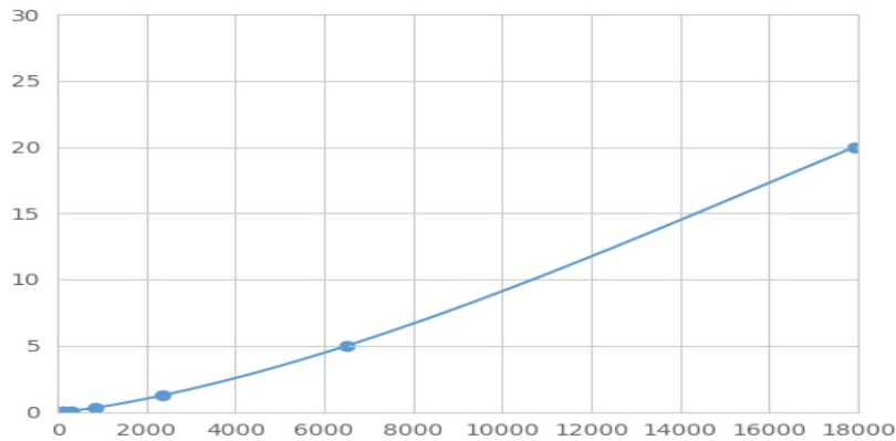
Typical Standard Curve for FKBPL Magnetic Luminex Assay.
