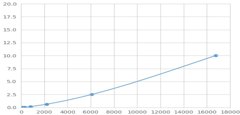
Typical Standard Curve for FAM132A Magnetic Luminex Assay.
