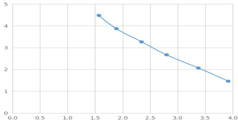
Typical Standard Curve for FPA Magnetic Luminex Assay.
