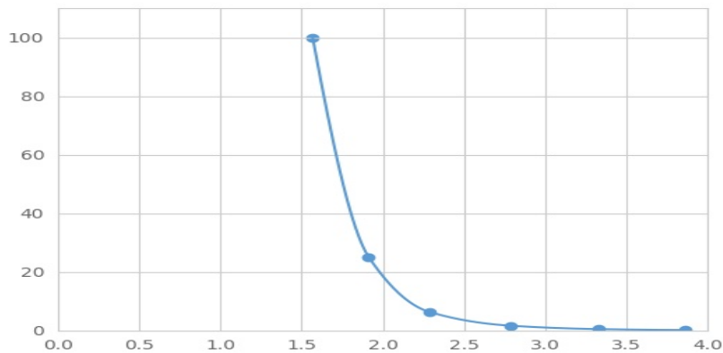
Typical Standard Curve for FPB Magnetic Luminex Assay.
