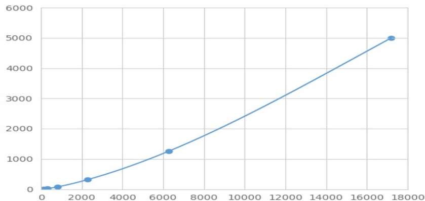
Typical Standard Curve for FLII Magnetic Luminex Assay.
