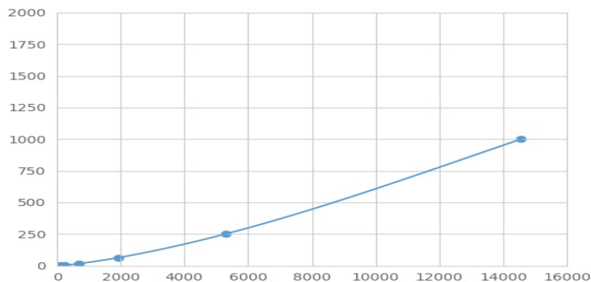
Typical Standard Curve for FSTL3 Magnetic Luminex Assay.
