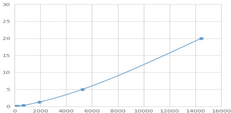
Typical Standard Curve for FZD6 Magnetic Luminex Assay.
