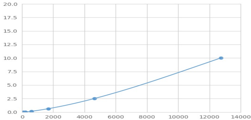
Typical Standard Curve for FUS Magnetic Luminex Assay.
