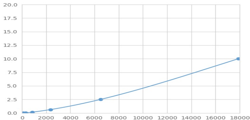
Typical Standard Curve for GSK3a Magnetic Luminex Assay.
