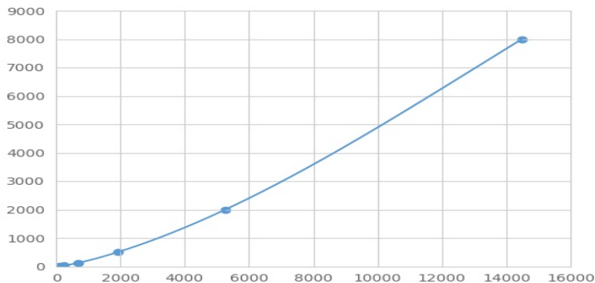
Typical Standard Curve for gp130 Magnetic Luminex Assay.
