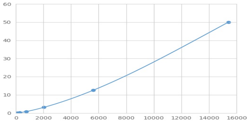
Typical Standard Curve for GPC1 Magnetic Luminex Assay.
