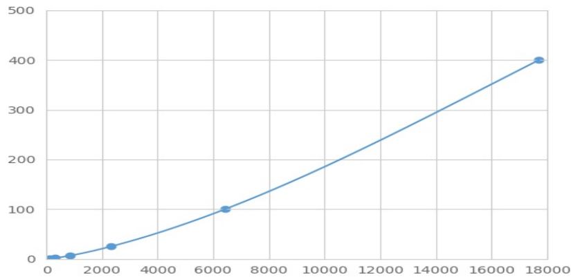
Typical Standard Curve for Hpt Magnetic Luminex Assay.
