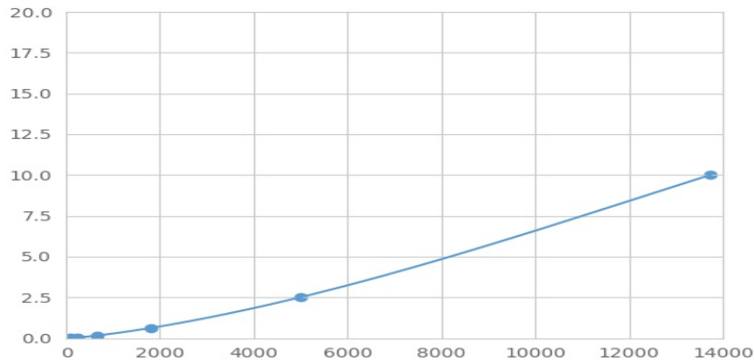
Typical Standard Curve for HRSP12 Magnetic Luminex Assay.
