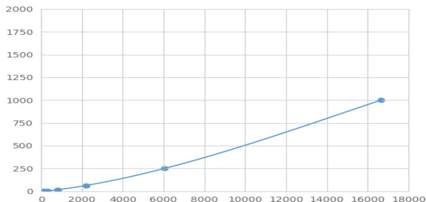
Typical Standard Curve for HSPb2 Magnetic Luminex Assay.
