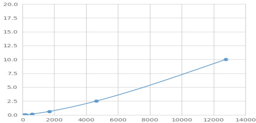
Typical Standard Curve for IHH Magnetic Luminex Assay.
