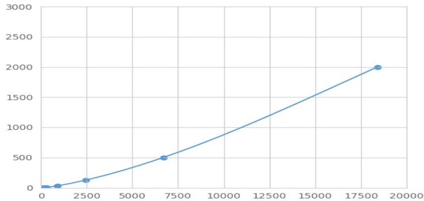
Typical Standard Curve for HO1 Magnetic Luminex Assay.
